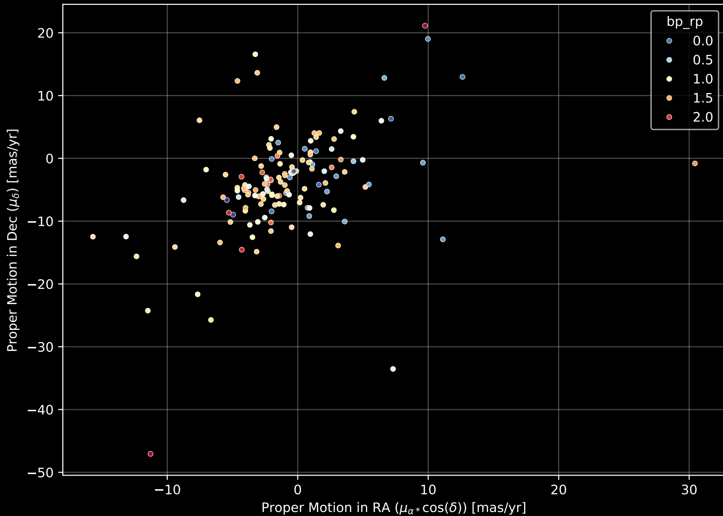
APOGEE DR17 Field: [N6791] Proper Motion Diagram (n= 165)
