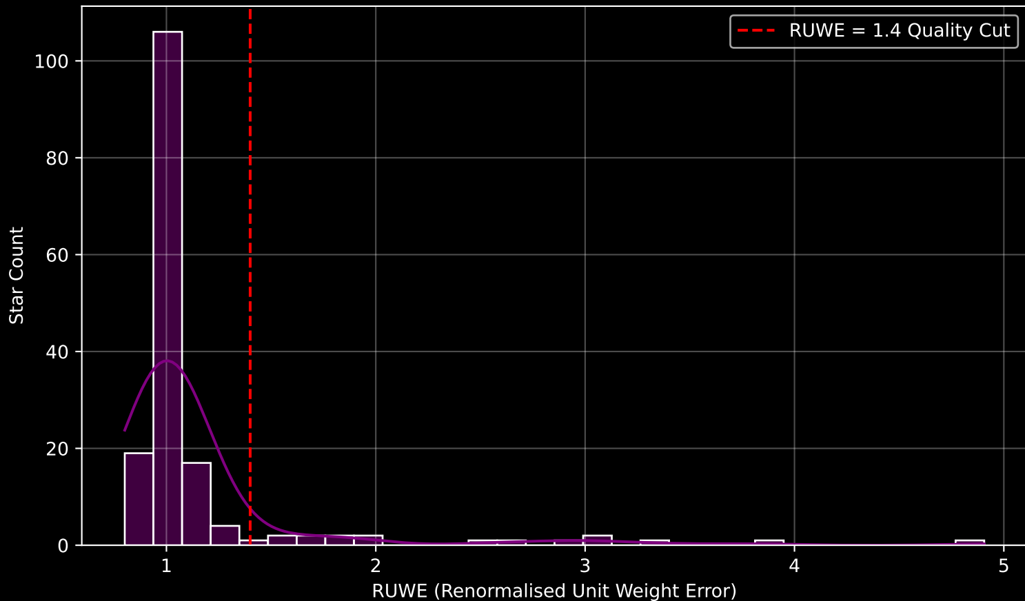
GAPOGEE DR17 Field [N6791] RUWE Distribution (n= 163)
