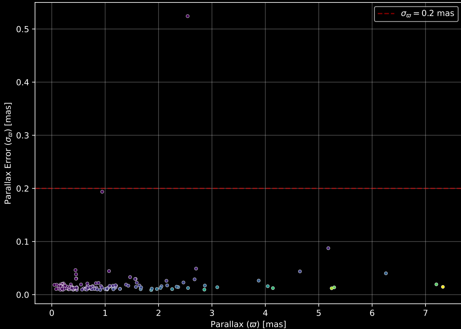
APOGEE DR17 Field: [N6791] Parallax Quality (n= 165)
