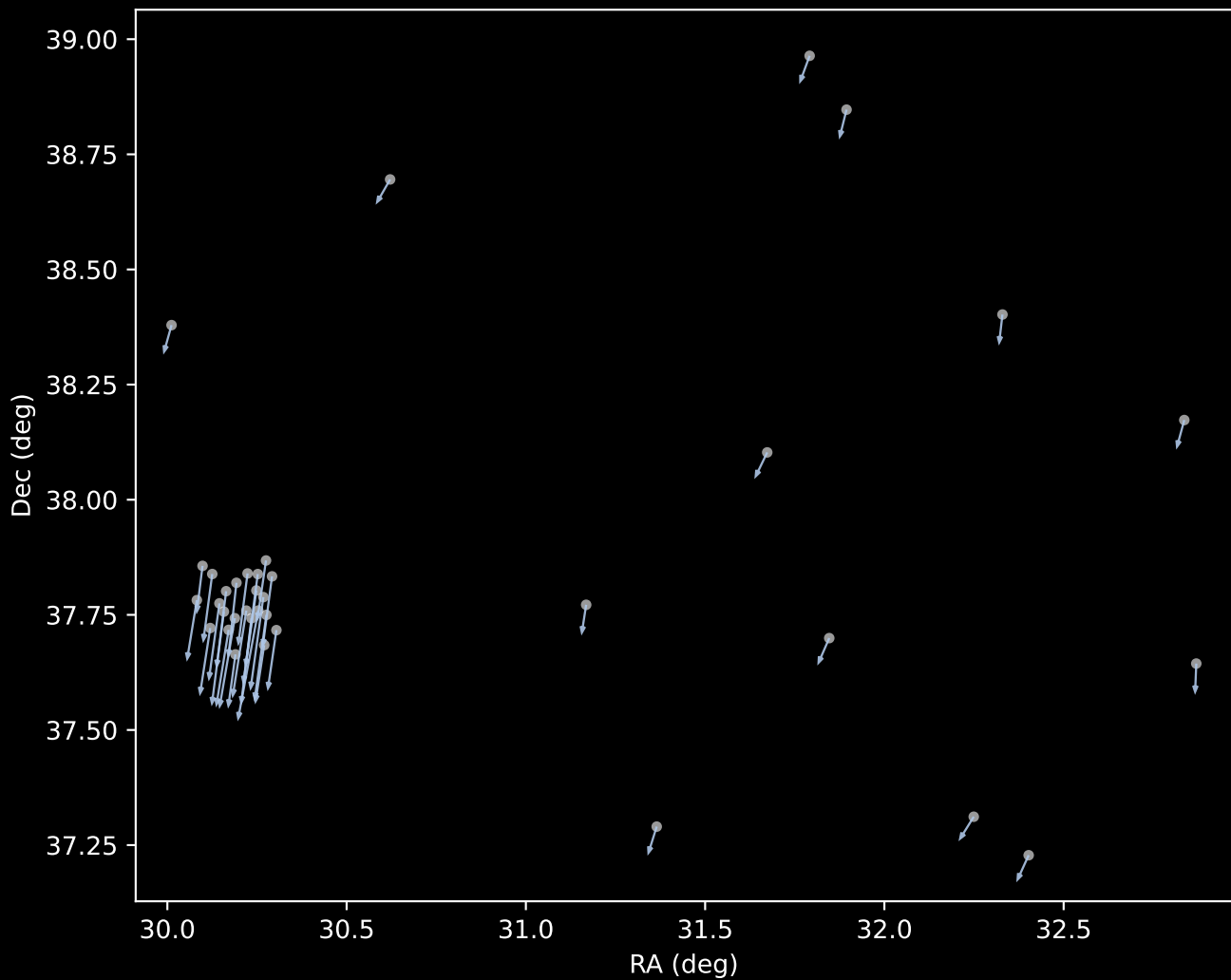
APOGEE DR17 Cluster 1 Proper Motion Vectors (n=36)
