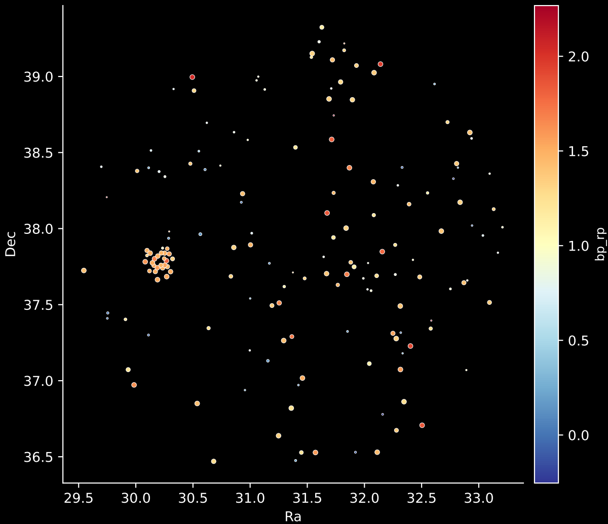
APOGEE DR17 Field: [N6791] Stars: 165
