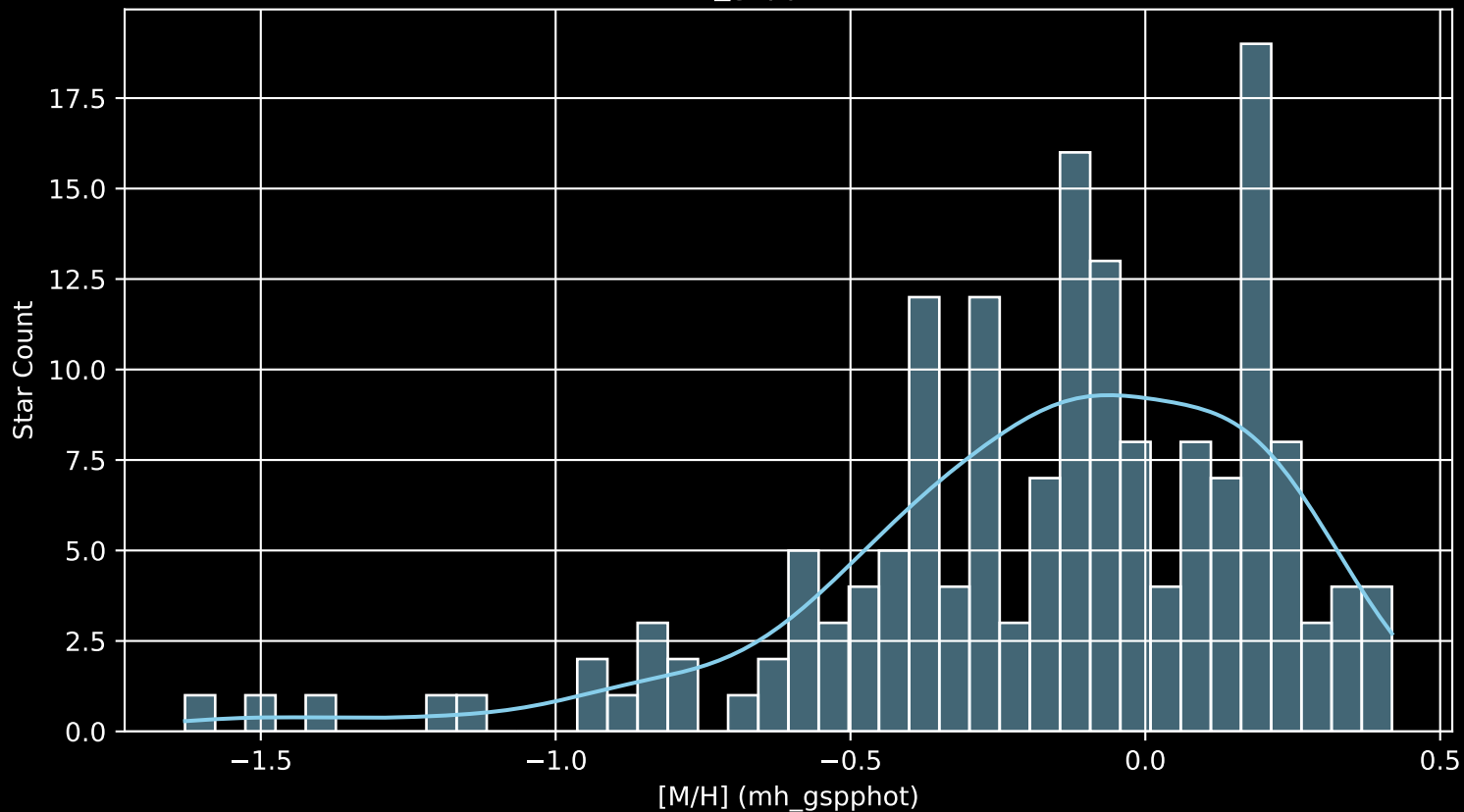
APOGEE DR17 Field: [N6791 [M/H] (mh_gspphot) (n= 165)
