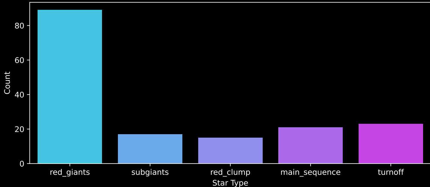
APOGEE DR17 Field: [N6791] Count plot of Star Type
